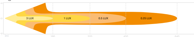
Lightbar FX500-SP
