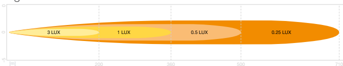
Lightbar FX250-CB
